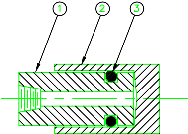
HEAD STEAM CYLINDER(No.27) (PART No.A-4240)
